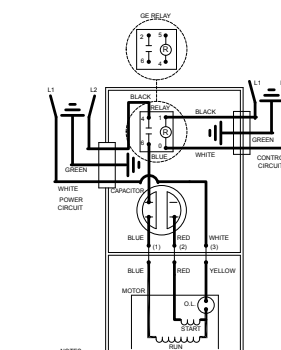
WIRING DIAGRAM FOR MODELS E405 & I405 ALL REVISIONS
