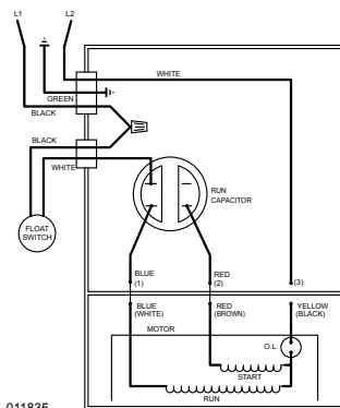
WIRING DIAGRAM FOR MODEL WD405 ALL REVISIONS
